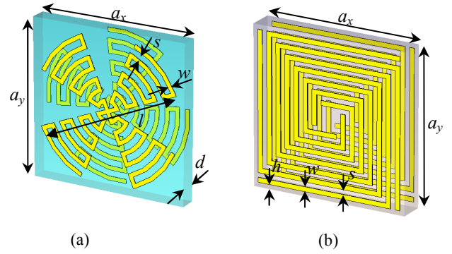
Fig. 3. (a) Unit cell of multi-turn cross wires CMM structure. The geometric parameters are given by a_x = a_y = 15 \text{ mm} , l = 14.4 \text{ mm} , w = 0.4 \text{ mm} and s = 0.6 \text{ mm} , d = 1.6 \text{ mm} . (b) Unit cell of four-arm spiral CMM structure. The geometric parameters are given by a_x = a_y = 10 \text{ mm} , d = 1.6 \text{ mm} , w = s = h = 0.3 \text{ mm} . The FR-4 board with dielectric constant of 4.5, dielectric loss tangent of 0.025 is utilized.
