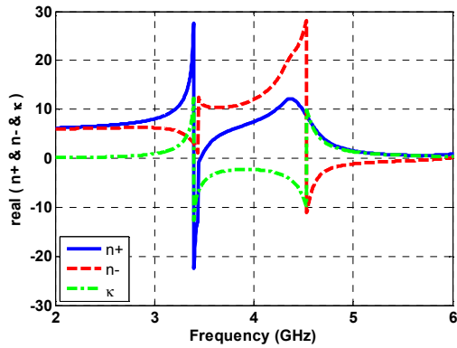
Fig. 2. The real parts of the RCP and LCP refractive indices and the chirality parameter of dendritic fractal CMM structure.
