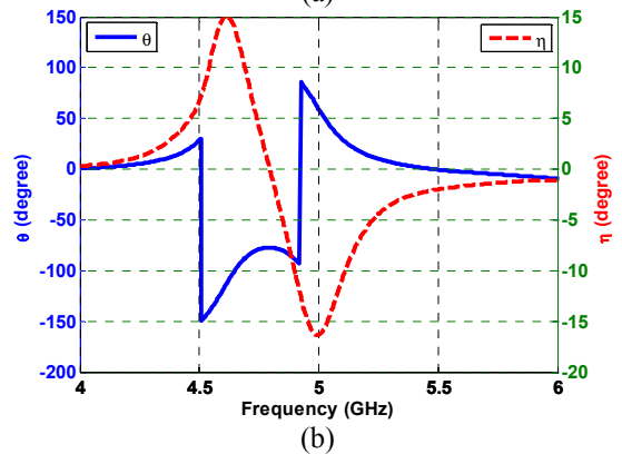
Fig. 4. (a) The real parts of the RCP and LCP refractive indices and the chirality parameter of multi-turn cross wires CMM structure. (b) The polarization azimuth rotation angle \theta and the ellipticity angle \eta of the four-arm spiral CMM structure.
