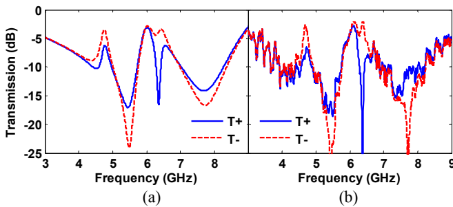
Fig. 6. (a) Simulation and (b) experimental results of the transmission coefficients for the dual-band CMM structure.
