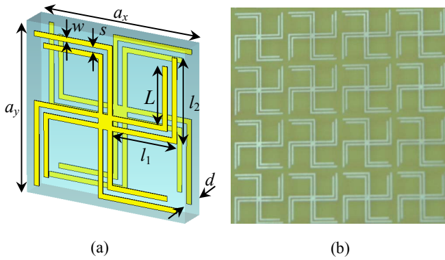
Fig. 5. (a) Schematic representation of a unit cell of the dual-band CMM structure. (b) Photograph of the experimental sample. The geometric parameters are given by a_x = a_y = 10 mm, L = 3.45 mm, l_1 = 4.05 mm, l_2 = 4.95 mm, w = s = 0.3 mm and d = 1.6 mm.
