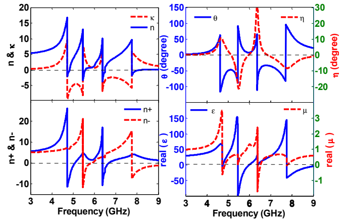
Fig. 7. The real parts of the refractive index n and \kappa for the dual-band CMM structure.
