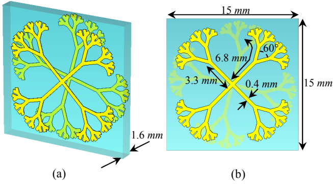
Fig. 1. (a) Perspective view of the unit cell of dendritic fractal CMM structure; (b) top view of the unit cell structure with its geometric parameters. The FR-4 board with dielectric constant of 4.5, dielectric loss tangent of 0.025 is utilized.
