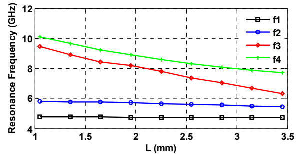
Fig. 8. The variations of resonant frequencies of the dual-band CMM structure with parameter L .
