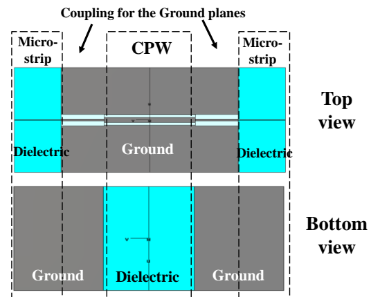
Figure 6: Microstrip to CPW conversion unit.
