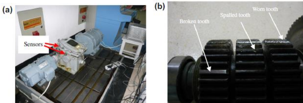
Fig3. (a) The gear fault test setup (Sepahan Cement), and (b) the appearance of the faulty gears.
