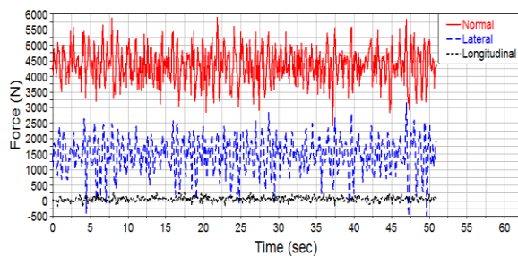
Figure 7: Test No. 3 - Load time histories
