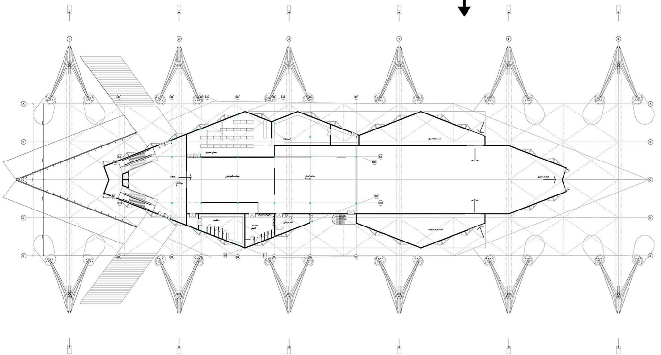
Ground Floor Plan Scale 1:200
