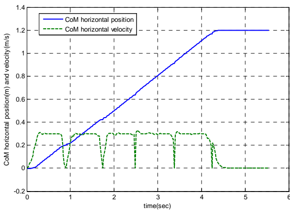
Fig. 4. Horizontal position and velocity of CoM with slow varying disturbances.
