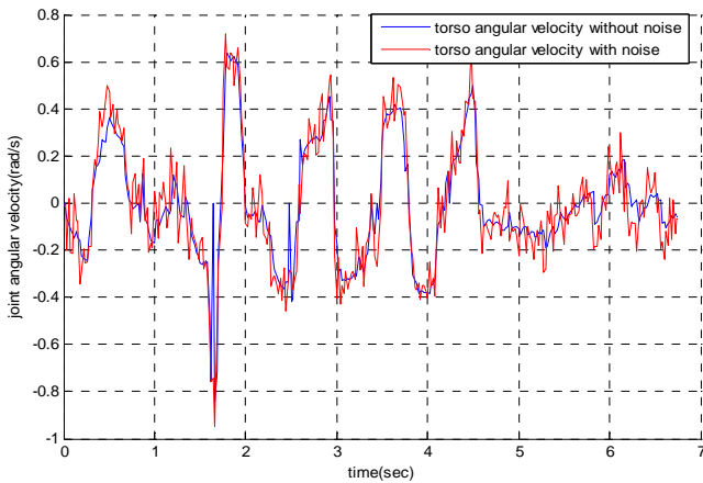
Fig. 9. Torso angular velocity with and without measurement noise.
