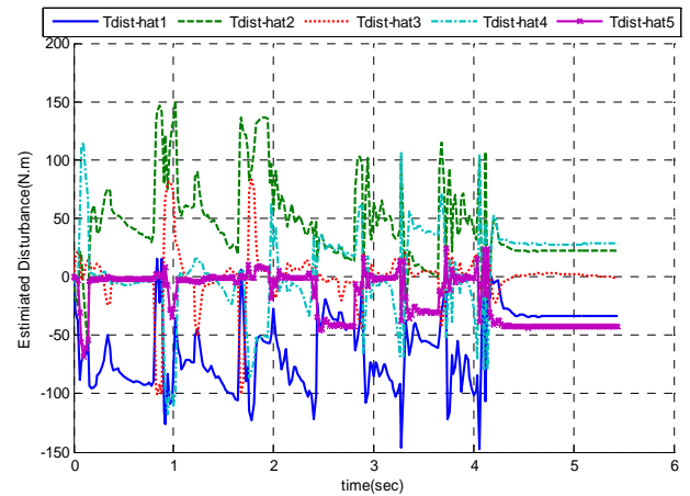
Fig. 7. Estimated disturbance torques.
