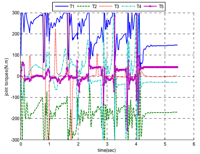
Fig. 6. Joint torques.
