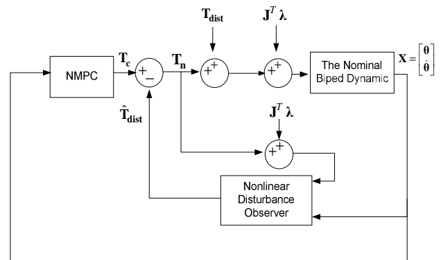
Fig. 3. Block diagram of the control method including NDO
