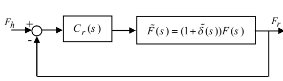
Figure 9. The equivalent block diagram of Figure 8.
