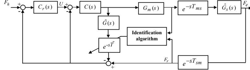
Figure 11. The structure design against model mismatch.
