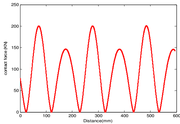
Fig10. contact force for wheel with velocity of 100 Km/h
