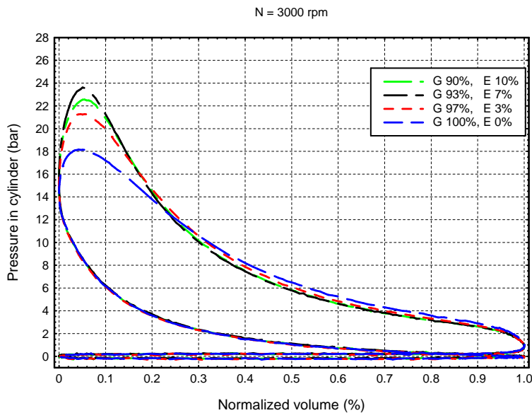
Fig.9. P-V Diagram
