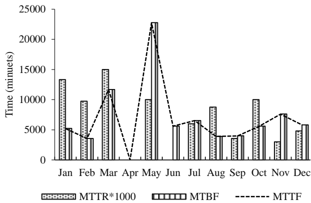
Figure 6. Estimation of MTTR, MTBF, and MTTF for Peugeot assembly line
