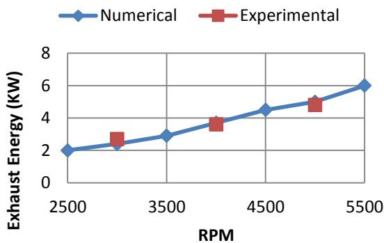
Figure 5: Exhaust Temperature Validation of Engine
