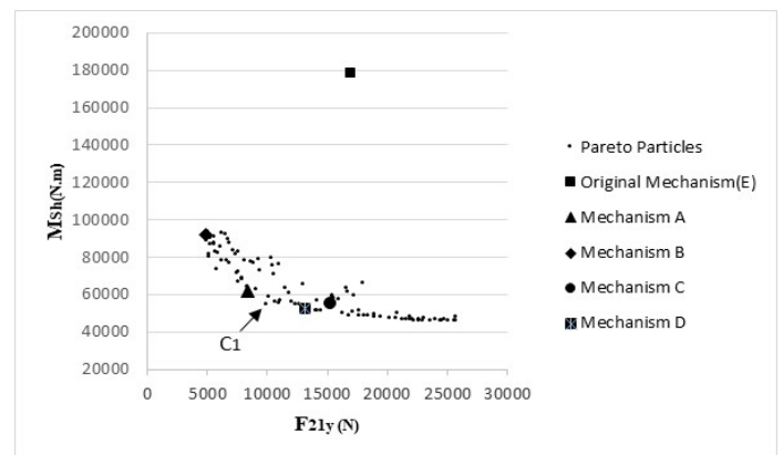
Figure 9: Pareto front of F_{21y} and M_{sh}
