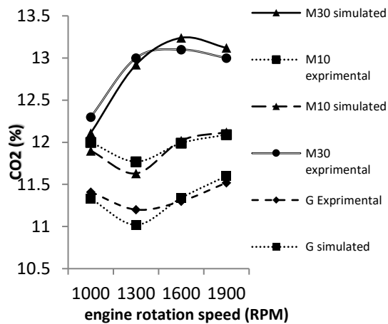
Figure 15. CO 2 emissions Changes in engine speed at different percentages of methanol
