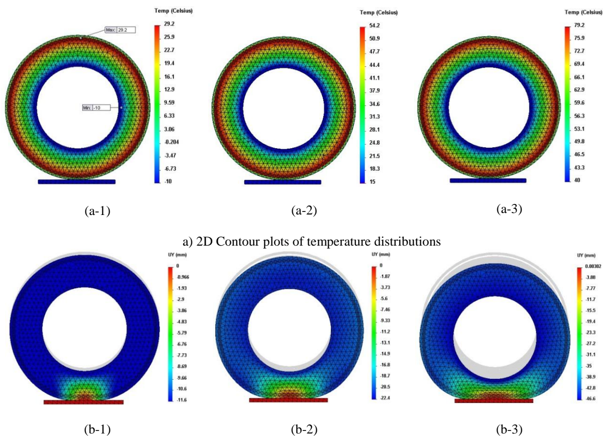
b) Maximum displacement contours of the tire at 10 th time step
