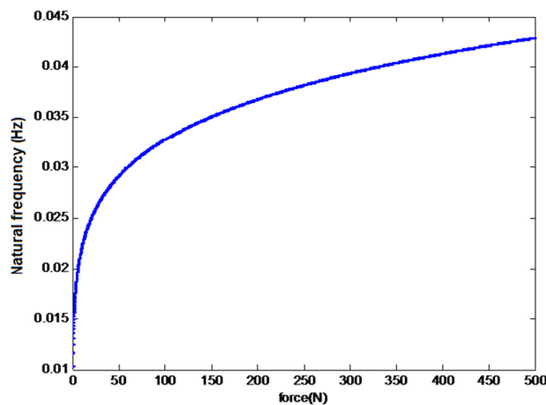
Fig7. Dependency of frequency on the preload
