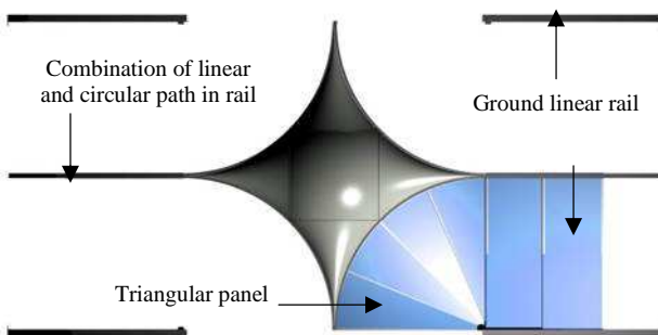
Fig. 11. Four triangular and two rectangular panels of each deployable section with two different rails
