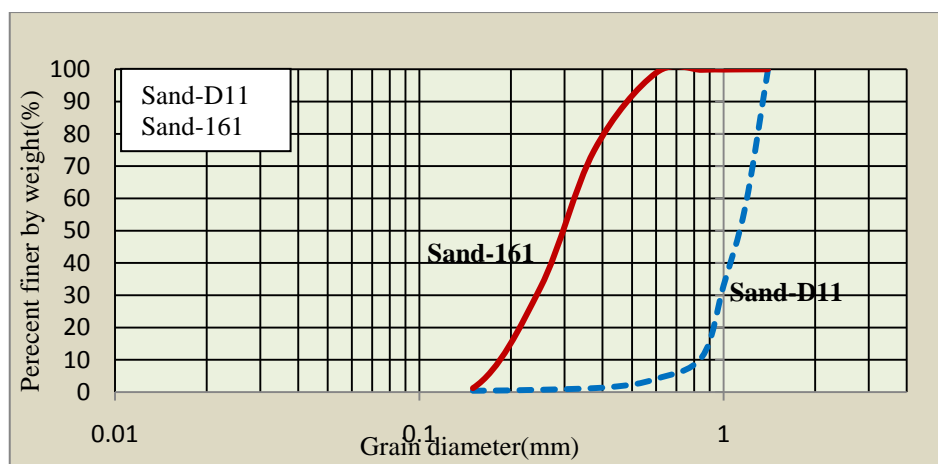
Fig. 1 Gradation curve for sand No 161 and D11 Firuzkough
