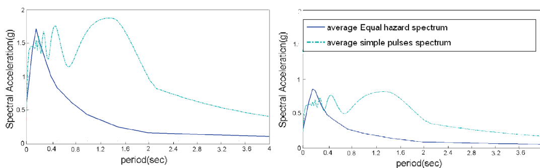
Fig. 10. Average pulse model spectrum are compared to equal hazard spectrum in the sites at one (left) and ten (right) kilometers of North-Tabriz Fault, for %10 probability of exceedance in 50 years
