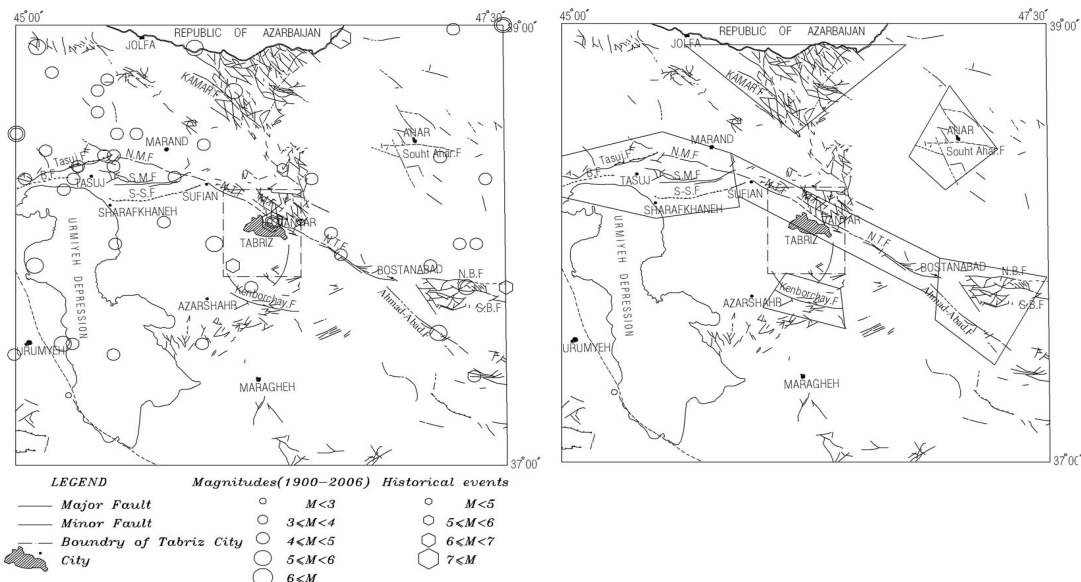
Fig. 2. a) Map of tectonic elements and seismicity in the Tabriz region. b) Potential area sources selected for seismic hazard assessment.
