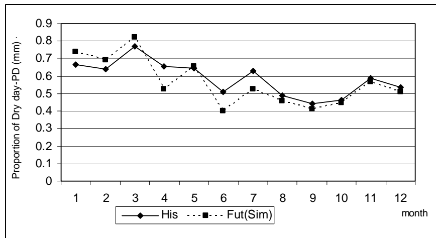
Figure 3. Summary statistics (MDR and PD) for 25 simulated sequences (FUT(SIM)) compared to historic (HIS) for Kassilian catchment rainfall (Oct.=Month 1)
