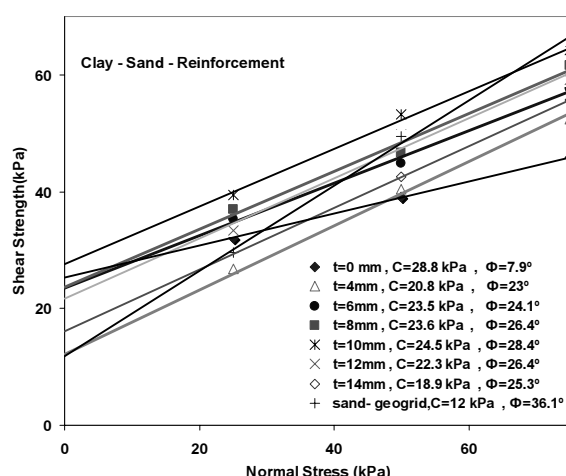
Fig. 9. Failure envelopes for clay – reinforcement, sand-reinforcement and Clay – sand - reinforcement samples
