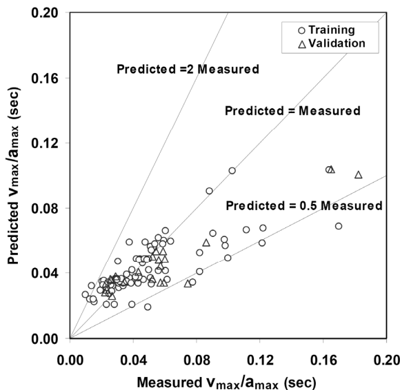
Fig. 6. The values of the v_{max}/a_{max} ratio predicted by GP versus the corresponding actual values for normal faulting mechanism
