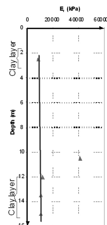
Fig. 5. Reload Moduli Vs Depth
