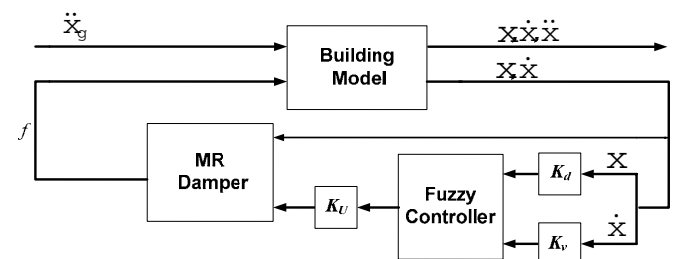
Fig. 6. control strategy of structure
