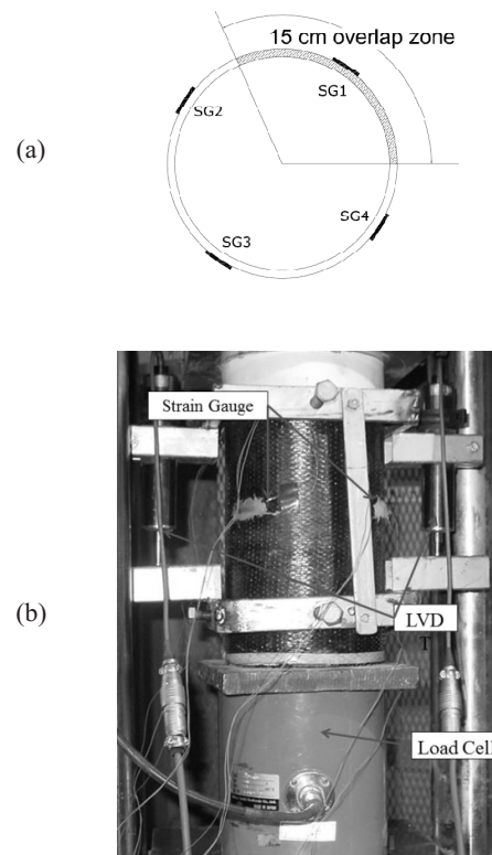
Fig. 1. (a) Strain gauges layout; (b) test specimen
