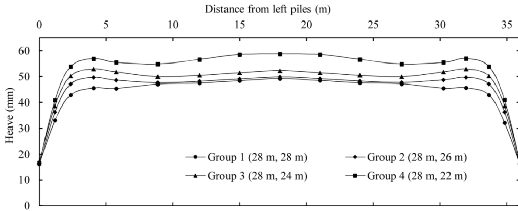
Fig. 7 Bottom heave under various pile lengths
