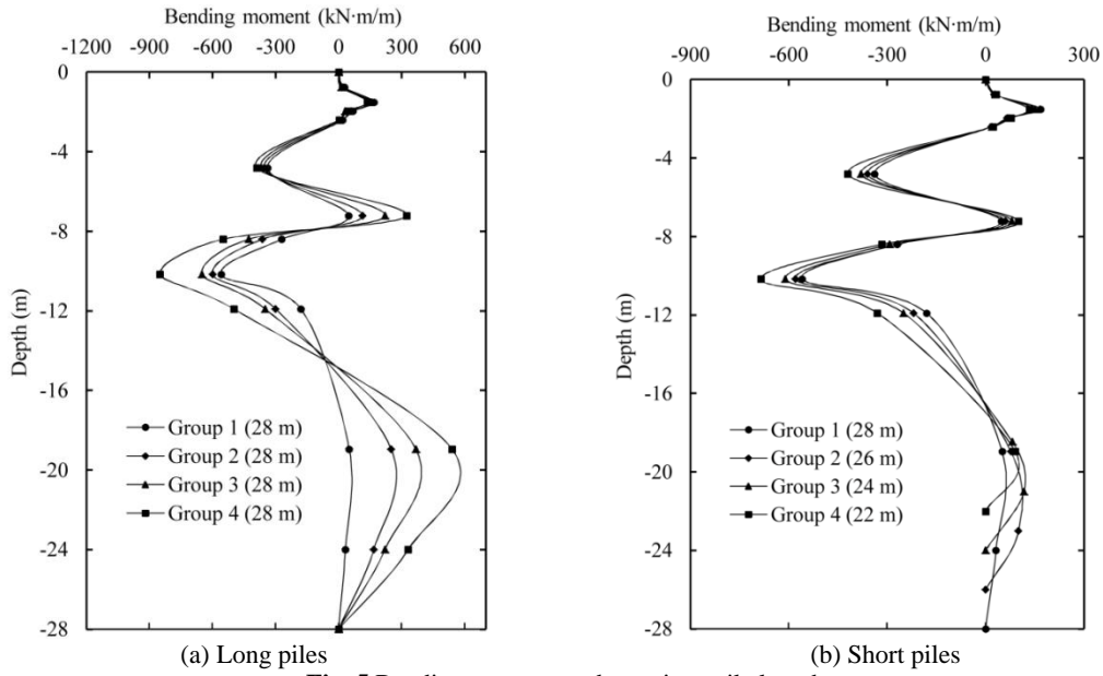
Fig. 5 Bending moment under various pile lengths
