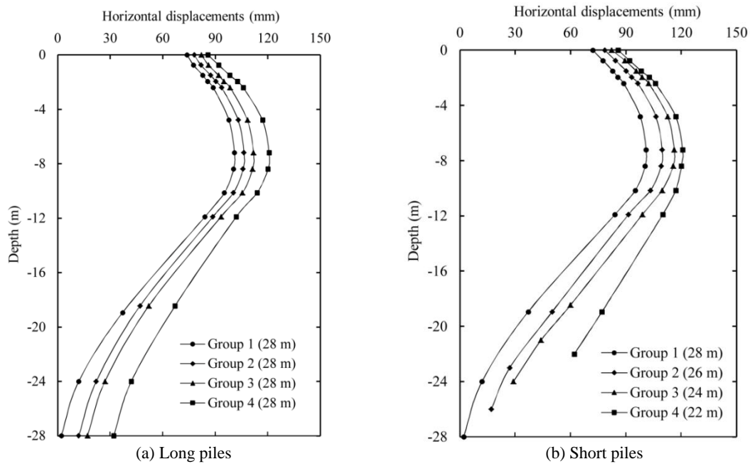
Fig. 6 Horizontal displacement under various pile lengths
