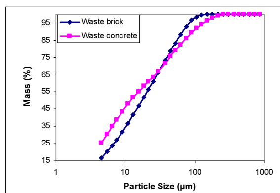
Fig. 1. Particle size distribution of ground waste brick and concrete
