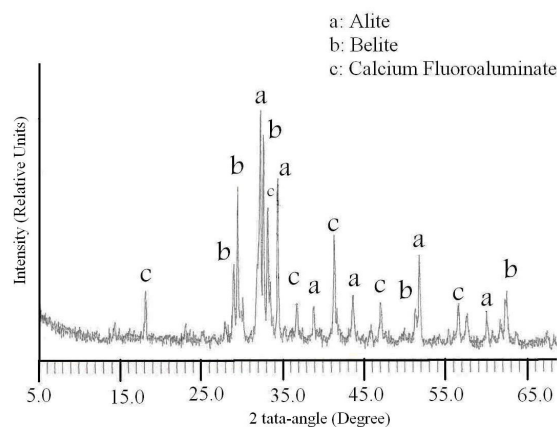
Fig. 5. X-ray diffraction pattern of clinker sample produced at 1270 °C
