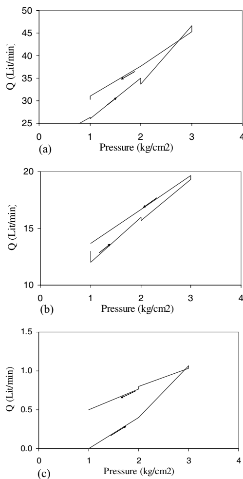
Fig.5 Water- Pressure tests for test hole S4. (a) Before injection, (b) After cement injection, (c) After cement and chemical injection
