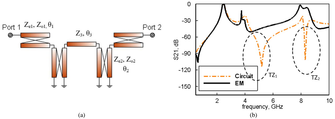
Fig. 2 a) Basic structure and b) Simulated results using ideal transmission-line models of proposed BPF.
