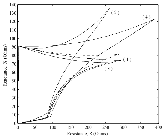
Fig. 21 Distance relay tripping characteristic variation; VT in front of, CT in front of UPFC.
