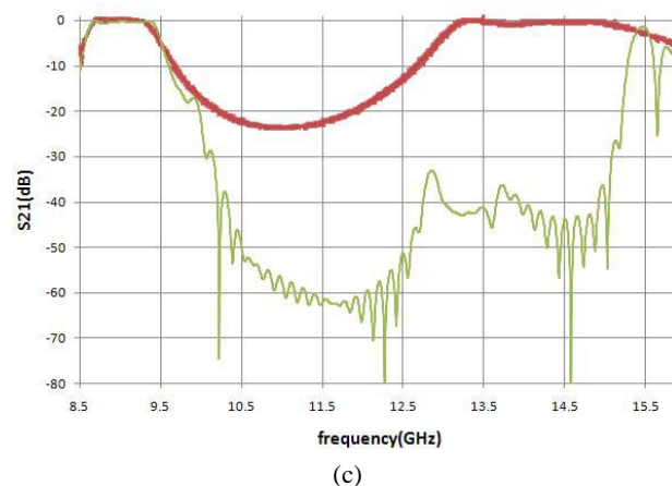
Fig. 5 (a), (b). The waveguide filter and the chiral array structure (c). The frequency response of the filter with improved out of band performance (green-thin line) compared to the original bandpass filter (red-thick line)
