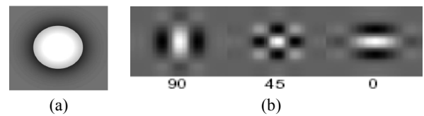
Fig. 2 (a) Input image. (b) 2-D impulse response of real wavelet transform to the input image at level 4 [34].
