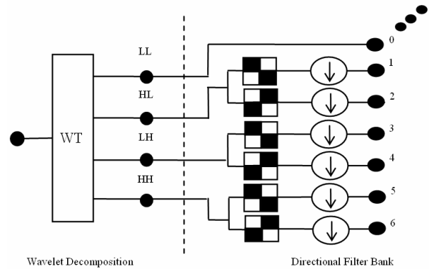
Fig. 1 1-level contourlet decomposition [42].
