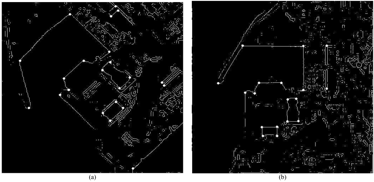
Fig. 7 Extracted corners from obtained edge map images (control points): (a) reference image, (b) sensed image.
