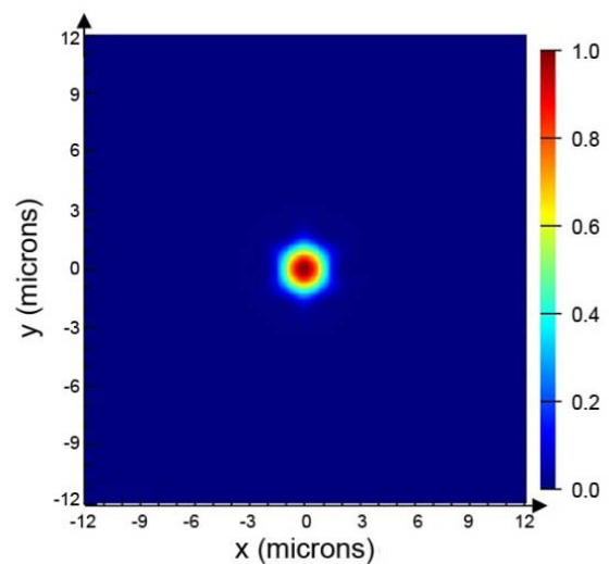
Fig. 5 Transversal field intensity distribution at a wavelength of \lambda = 1.55 \mu\text{m} for the fundamental guiding mode. d_1=d_2=6 \mu\text{m} and \Lambda=8 \mu\text{m} .
