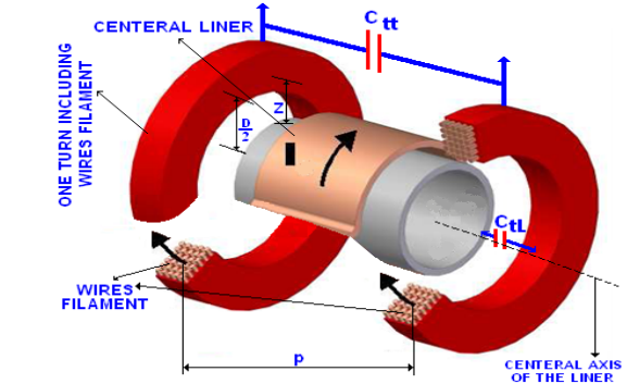
Fig. 13 Two adjacent turns which have k-CWF include circular cross-section, in the rectangular cross-section.
