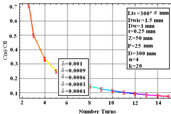
Fig. 21 Ratio of total capacitance of n turns to turn-turn capacitance C(n)/C_{tt} for different value of \delta .
