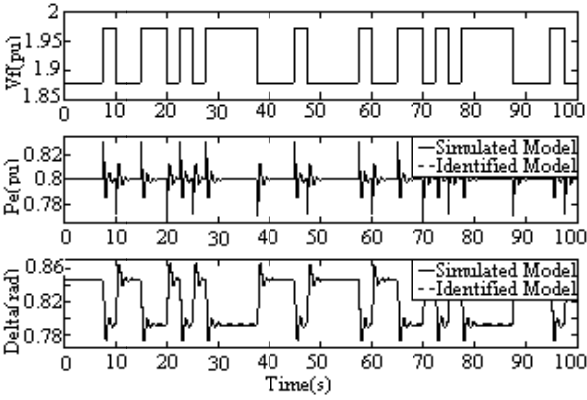
Fig. 3 data collected at operating point P=0.8, Q=0, v_t=1.05 .
