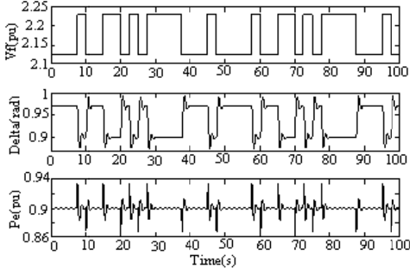
Fig. 2 data collected at operating point P=0.9, Q=0.1, v_t=0.98 .
