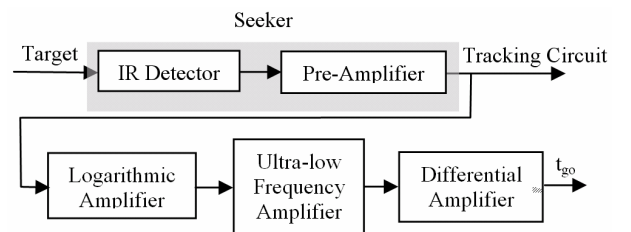
Fig. 3 Practical implementation for t_{go} calculation.
