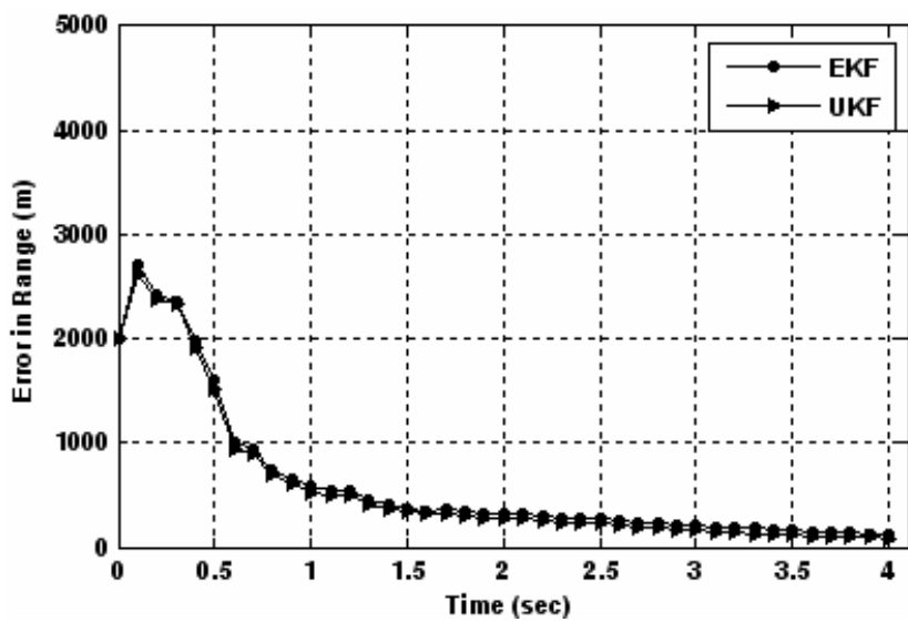
Fig. 6 Errors of the estimated range in scenario 3.
