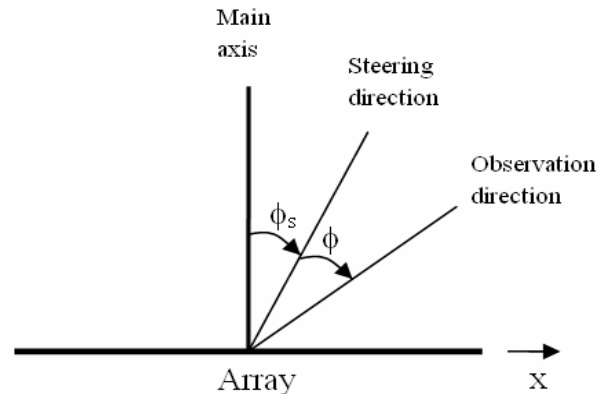
Fig. 1 The geometry showing steering and observation directions.
