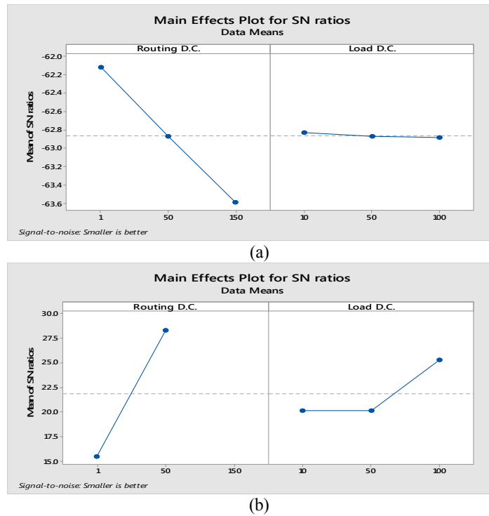
Fig. 8. Main effects plot at SN ratios. (a) response is total cost; (b) response is total deviation
