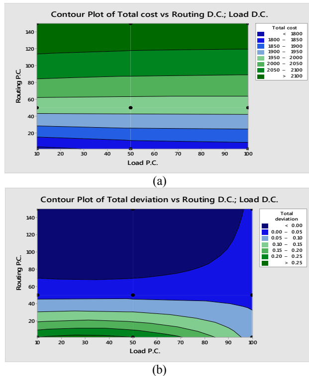
Fig. 9. Contour Plots, (a) Total cost vs Routing P.C. and Load P.C. (b) Total deviation vs Routing P.C. and Load P.C.
