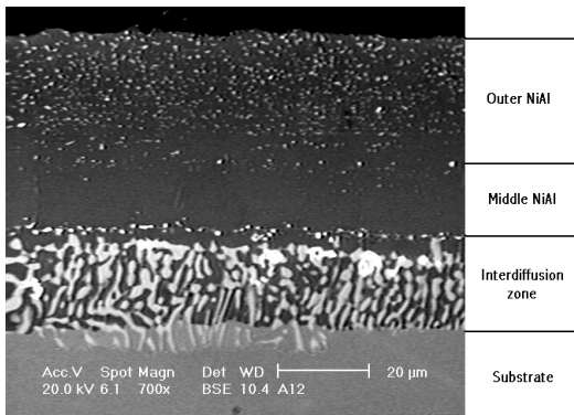
Fig. 4. Typical microstructure of silicon modified-aluminide, coating produced after heat treating the coated samples at 1030, 1050 and 1080°C for a period of either 4 or 8hrs.
