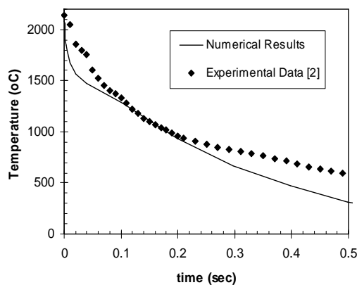
Fig. 9. Numerical temperature history curve in comparison with experimental data.
