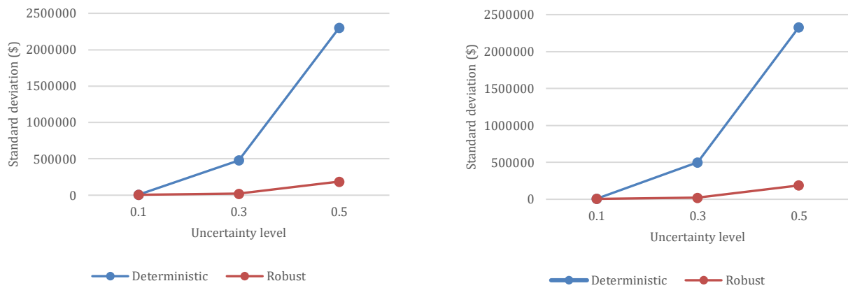
Fig. 5. Standard deviation of the OF values for \epsilon^1 (the left side) and \epsilon^2 (the right side)
