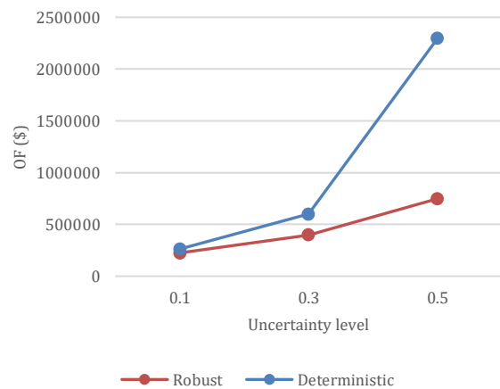
Fig. 4. Mean of the OF values for \varepsilon^1 (the left side) and \varepsilon^2 (the right side)
