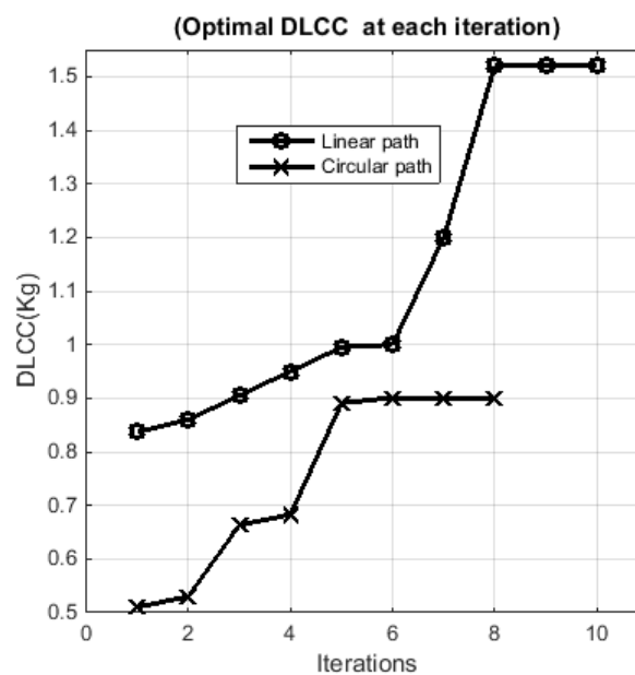
Fig. 5. Optimal dynamic load carrying capacity
