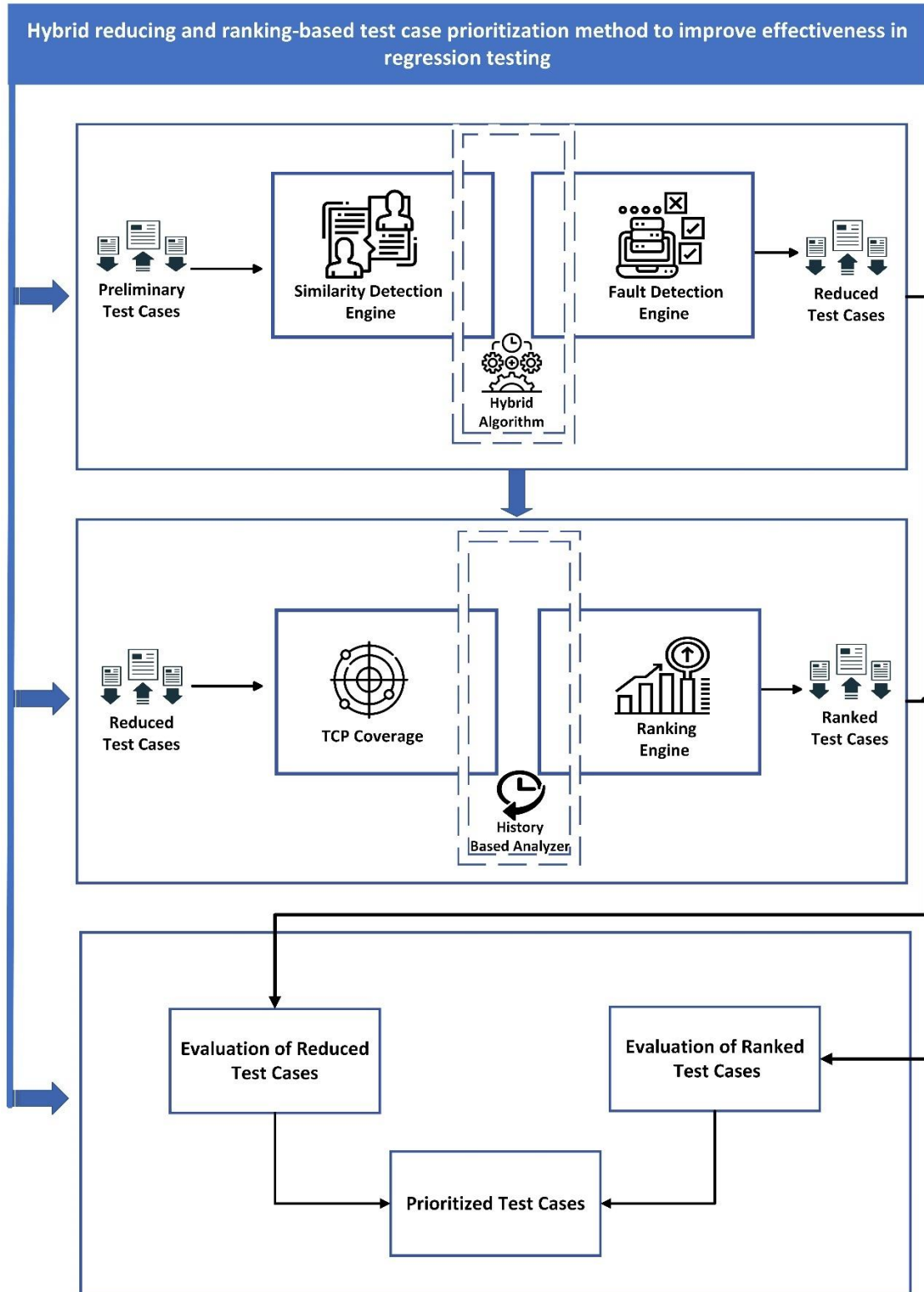
Fig. 2. Hybrid framework
