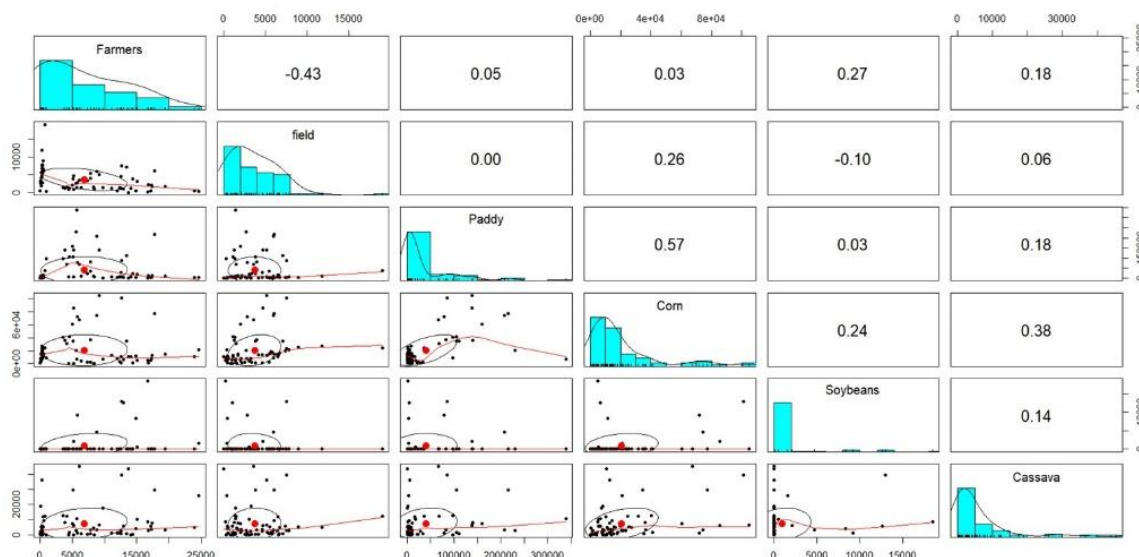
Fig. 2. Multicollinearity test
