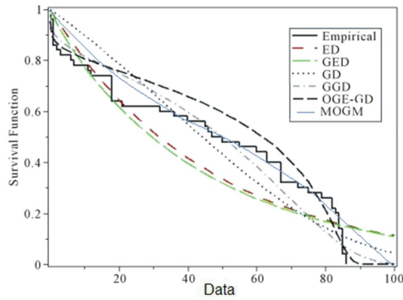
Fig. 6. Graph of survival function of compared distributions
