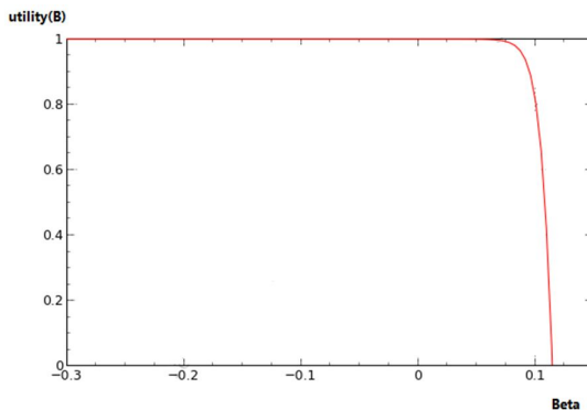
Fig.3. Illustrate DM's Risk utility (Beta)
