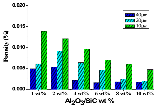
Fig. 7. The variation of porosity of the HMMCs with different weight fraction and particle size of Al_2O_3/SiC reinforcements
