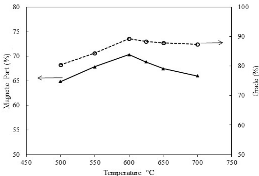
Fig.11. Effect of temperature on grade of product and the amount of magnetic part in different temperatures (roasting time: 25min, small particle size ore (180-250µm)).
