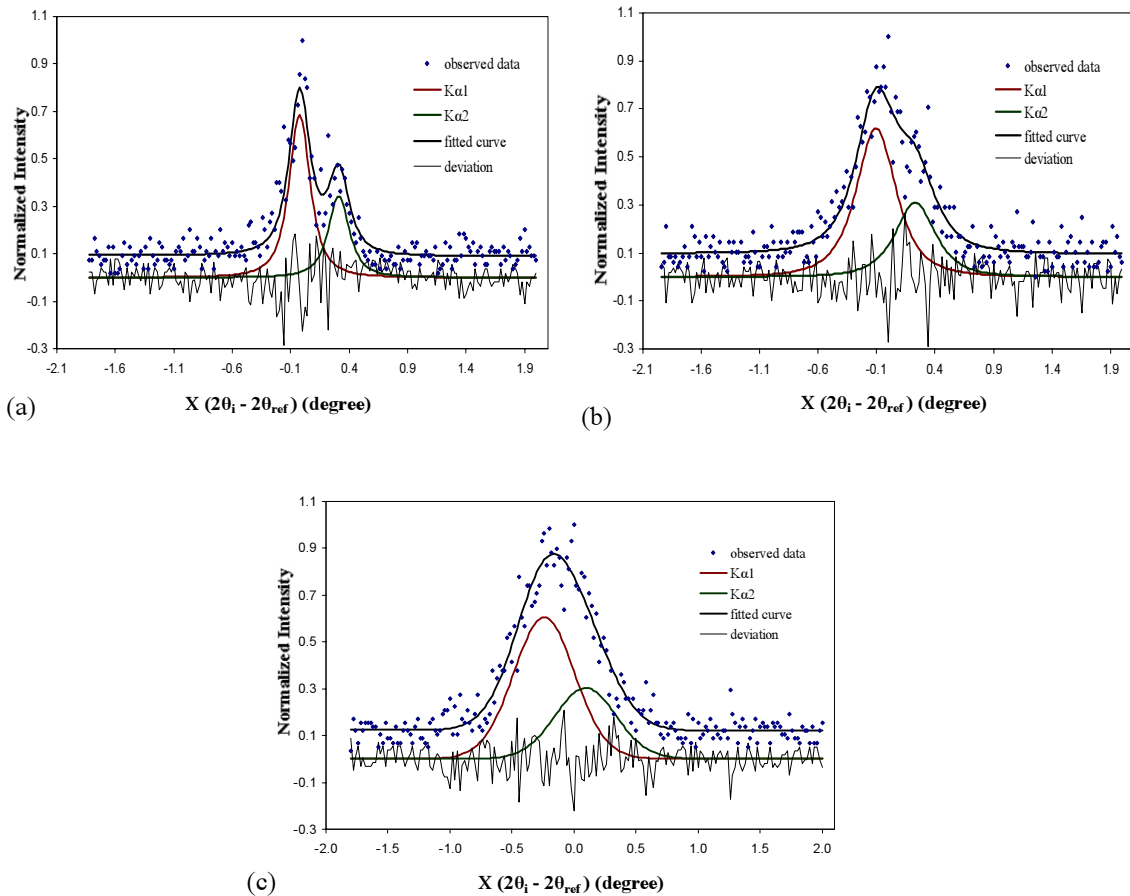
Fig. 2. The measured and fitted curve via Pearson function corresponding to the 400 reflections of Al: (a) before wear (b) 100N (c) 150N, the difference between the measured and the fitted values is also plotted in the lower parts.
