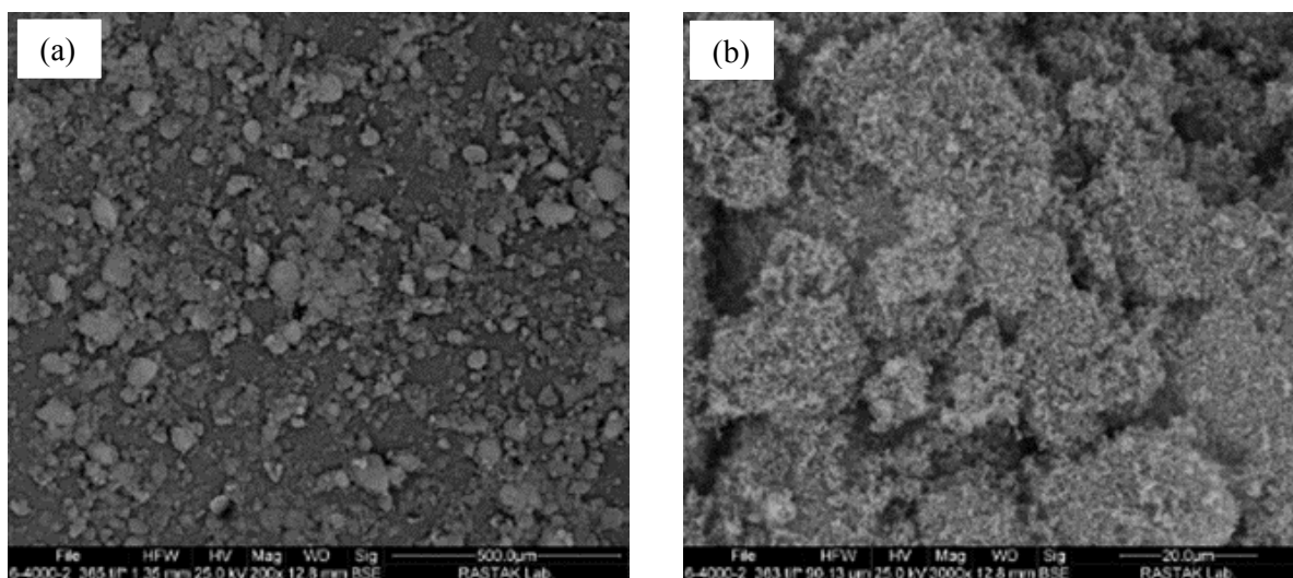
Fig. 10. SEM images of the coated surface by the synthesized hydrophobic nano-silica powder in the environment (a) surface with 500 μm magnifying and (b) the same surface with 20 μm magnifying.
