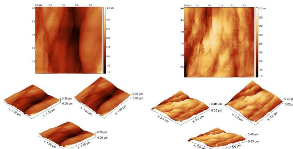
Fig. 12. The non-contact mode AFM images of the surface topography of the sample using the synthesized hydrophobic nano-silica powder.
